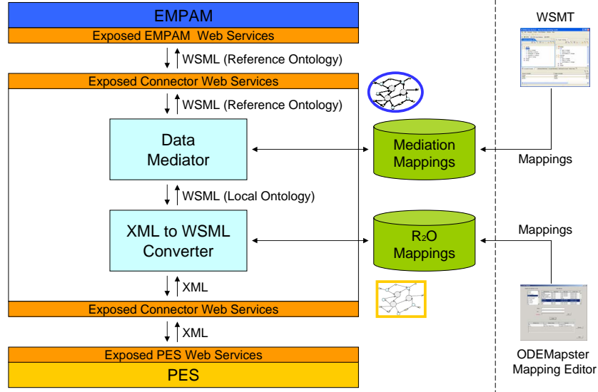
Fig. 5. The SEEMP Connector Architecture.
